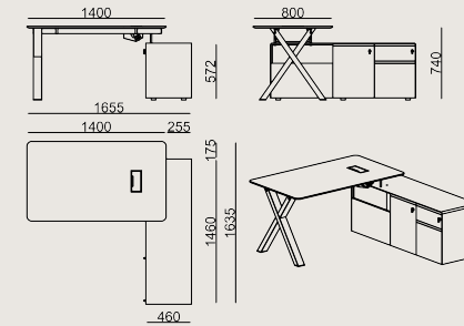
PARTITA S4 D0814RK LAMINATE_VENEER Overall Width: 1400 mm / 55.12" Overall Depth: 800 mm / 31.5" Overall Height: 740 mm / 29.13"
